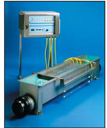
Scorpion® Series 8300 Open Channel Horizontal & Vertical Wastewater Ultraviolet Disinfection Systems
